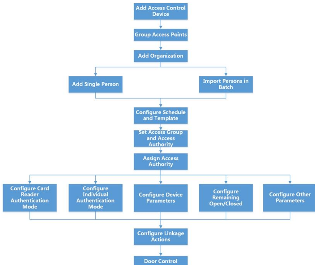
Figure 15-1 Flow Chart of Access Control
