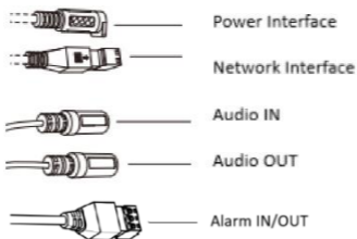
Figure 1-2 Overview of connectors
