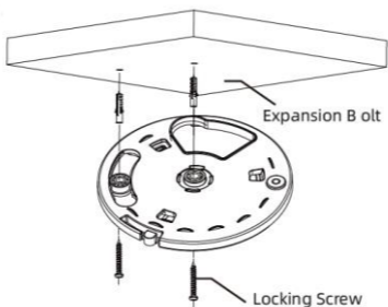
Figure 2-1 using the mounting base
