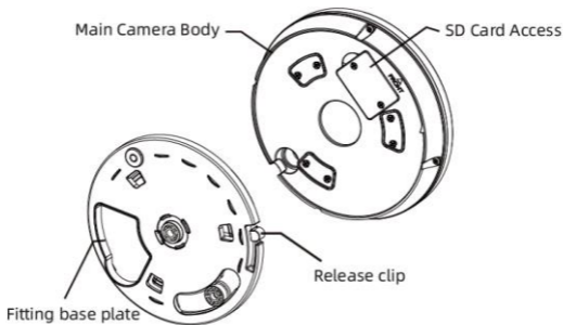
Figure 1-1 Overview of Fisheye Camera
