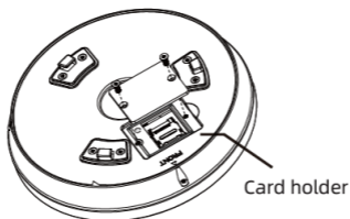
Figure 1-2 SD-card interface
