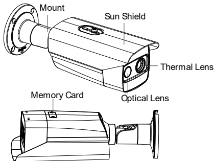
Figure 1-1 Overview of the Camera
