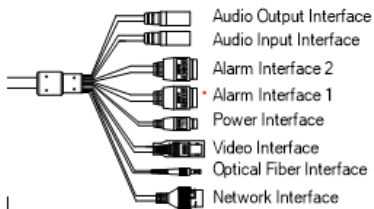
Figure 1-2 Cable Description
