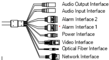
Figure 1-2 Cable Description
