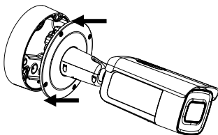
Figure 2-5 Remove the Junction Box
