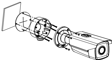
Figure 2-6 install the bracket
