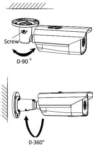
Figure 2-6 Adjust the View Angle
