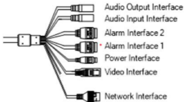
Figure 1-2 Cable Description
