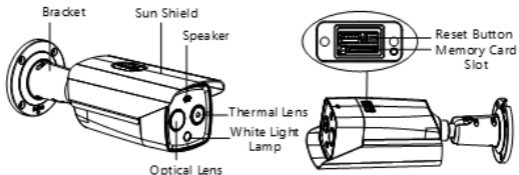
Figure 1-1 Overview of the Camera
