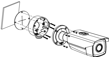
Figure 2-6 install the bracket
