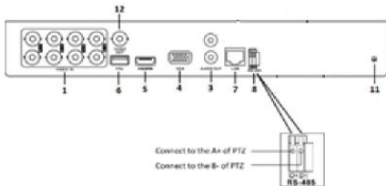
Figure 2-7 PTZ Connection
