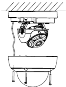
Figure 2-4 reinstall cover
