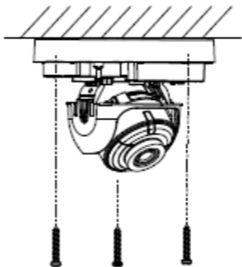
Figure 2-2 Fix the Camera on the Ceiling
