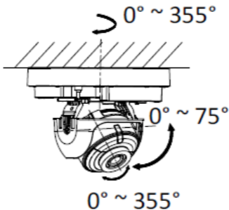
Figure 2-3 3-axis Adjustment
