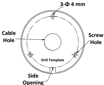
Figure 2-1 The Drill Template
