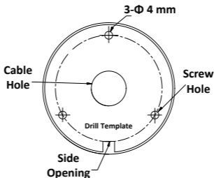
Figure 2-1 The Drill Template
