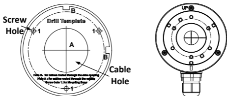
Figure 2-4 The Drill Template
