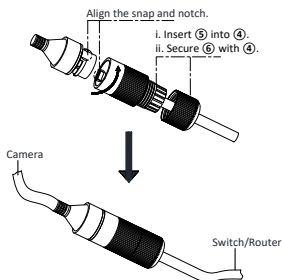
Figure 2-8 Water-proof Accessory Installation
