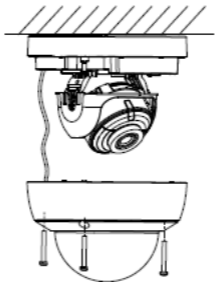
Figure 2-4 reinstall cover
