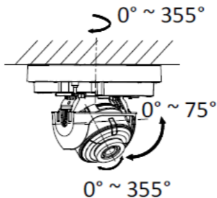
Figure 2-3 3-axis Adjustment
