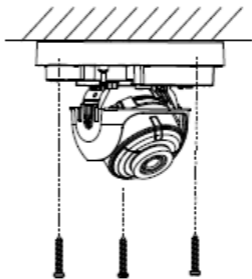
Figure 2-2 Fix the Camera on the Ceiling
