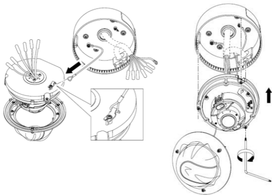
Figure 2-5 fix the safety rope
