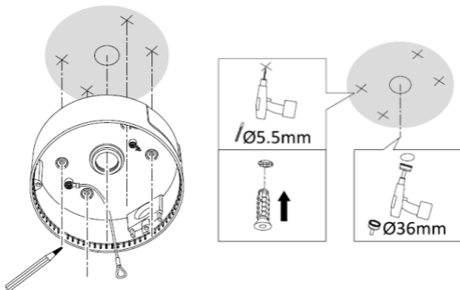
Figure 2-2 Drill Template
