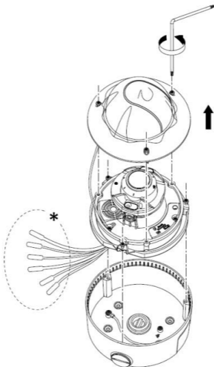
Figure 1-1 Overview of the Camera
