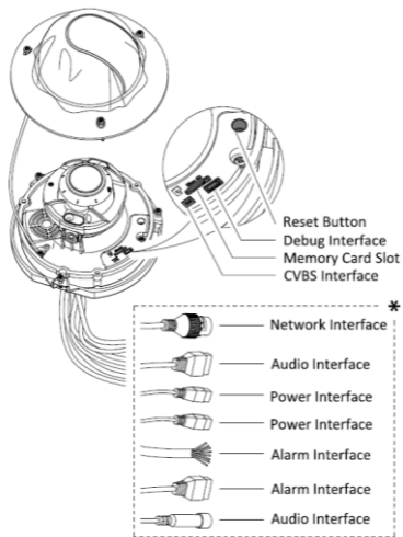
Figure 1-2 Cable Description
