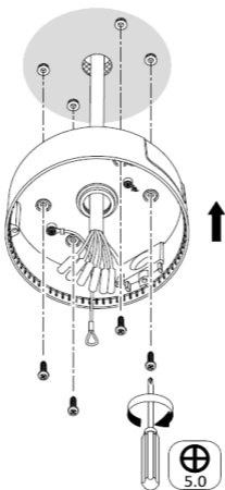
Figure 2-3 fix the camera base
