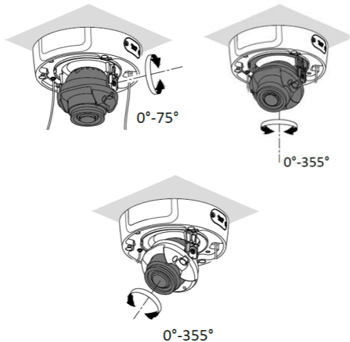
Figure 2-4 Adjust the View Angle
