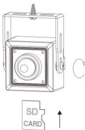
Figure 1.2 Install the SD-card
