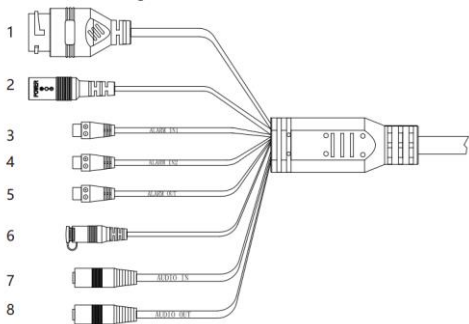
Figure 1-1 connections of camera
