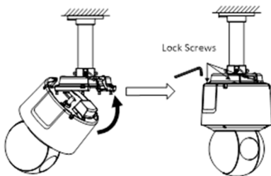
Figure 2-14 Finish the installation
