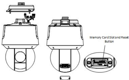
Figure 1-1 Overview of the IR Speed Dome
