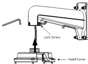
Figure 2-2 Install head cover
