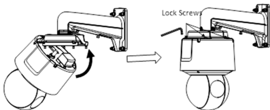
Figure 2-4 Secure the speed dome
