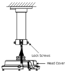
Figure 2-12 Fix the head cover
