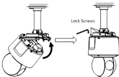
Figure 2-9 Finish the installation
