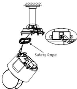
Figure 2-13 Use safe rope
