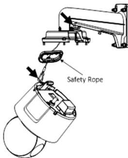
Figure 2-3 Use Safety Rope
