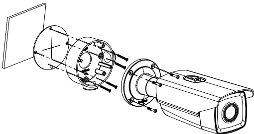
Figure 2-5 Install the Camera onto Junction Box
