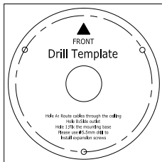
Figure 2-4 Drill Template
