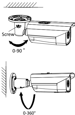
Figure 2-6 Adjust the View Angle
