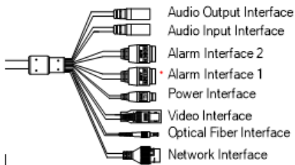
Figure 1-2 Cable Description
