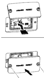
Figure 2-2. Insert the Memory Card
