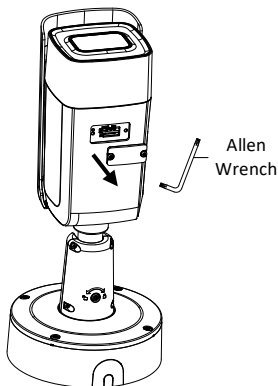
Figure 2-1 Remove the Cover of the Memory Card Slot
