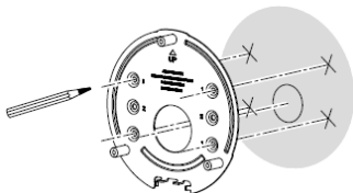
Figure 2-4 Drill Holes in the Wall/Ceiling
