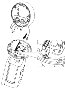
Figure 2-10 Hook the Camera to the Junction Box
