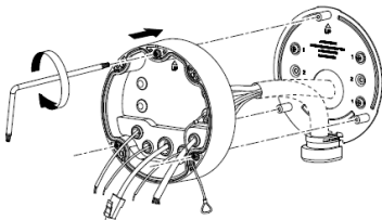
Figure 2-9 Secure the Junction Box
