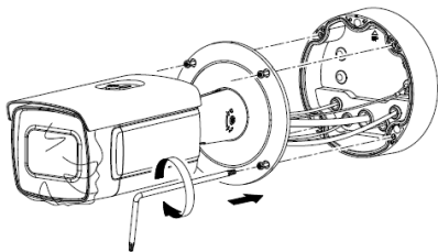
Figure 2-11 Secure the Camera
