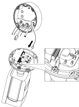
Figure 2-10 Hook the Camera to the Junction Box
