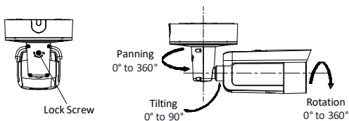
Figure 2-12 Adjust the View Angle
