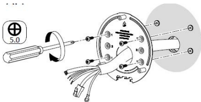
Figure 2-5 Install the Adapter
