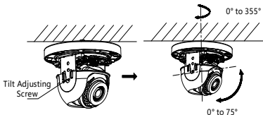
Figure 2-5 Type I Camera 2-Axis Adjustment
