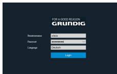
Figure 4-1 Login Interface
